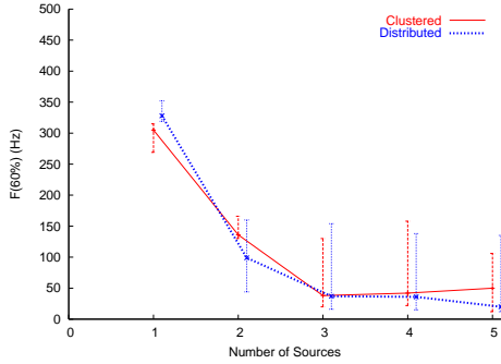
Figure 11: Localization of power as the number of sources increase in both clustered and distributed topologies. The error bars show 95% confidence intervals for the experiment.
