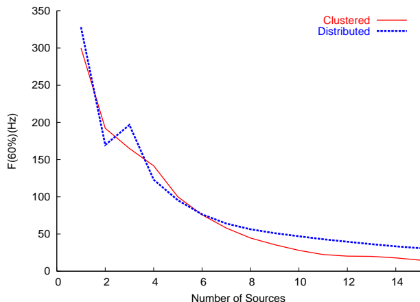
Figure 12: The effect of aggregation of multiple sources at different phases.
