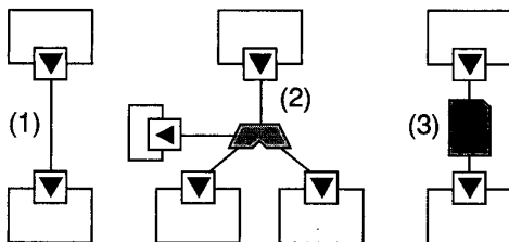
Figure 4. Koala's forms of binding
